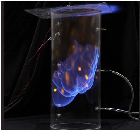
GAS IGNITION CHAMBER DEMONSTRATIONS
